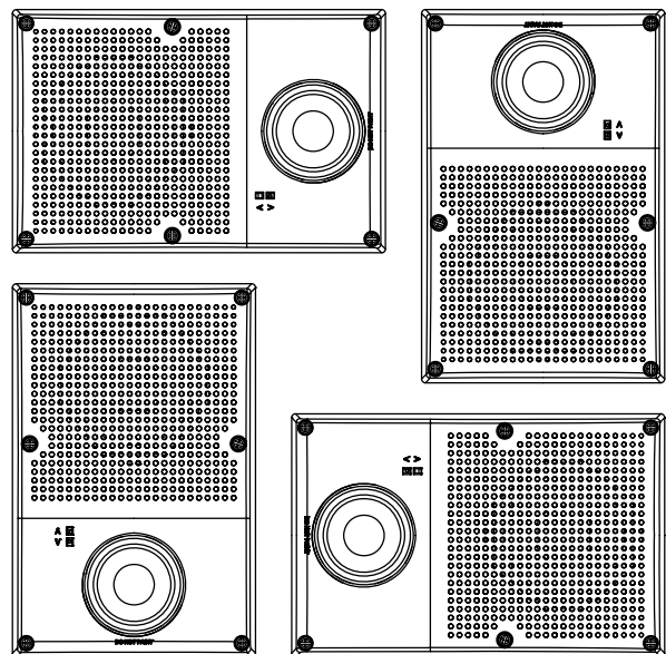
Figure 4: Mounting positions
