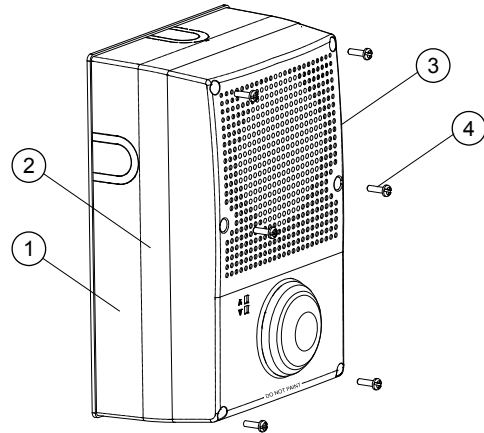
Figure 3: Assembled
