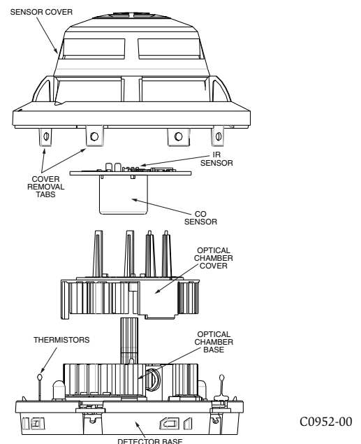
FIGURE 4. SENSOR ASSEMBLY:
