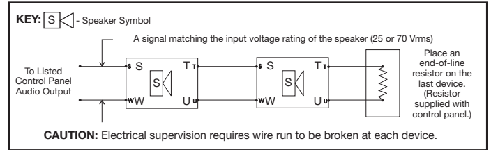
Figure 1: Wiring Diagram for Speaker
