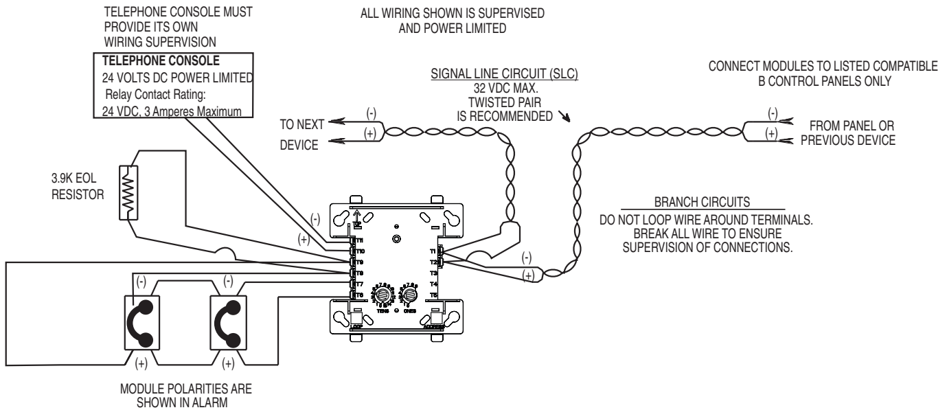
FIGURE 4. TYPICAL FAULT TOLERANT CIRCUIT CONFIGURATION, NFPA STYLE Z:
