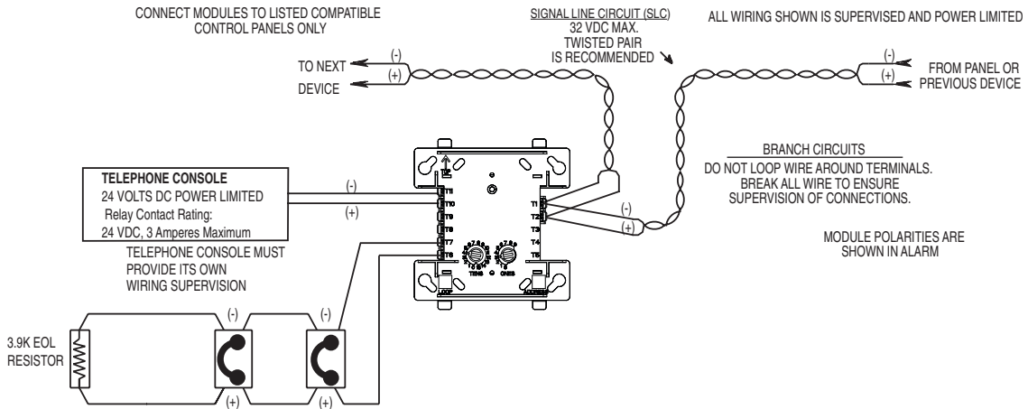
FIGURE 4. TYPICAL FAULT TOLERANT CIRCUIT CONFIGURATION, NFPA STYLE Z:
